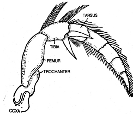
Natatorial leg
