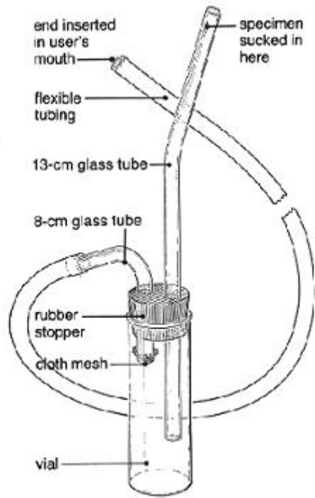
Aspirator/Potters/Suction tube
