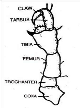
Scansorial leg
