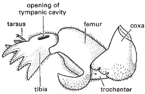
Fossorial leg
