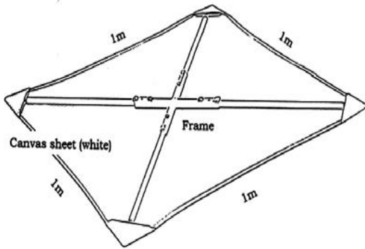
Beating tray
